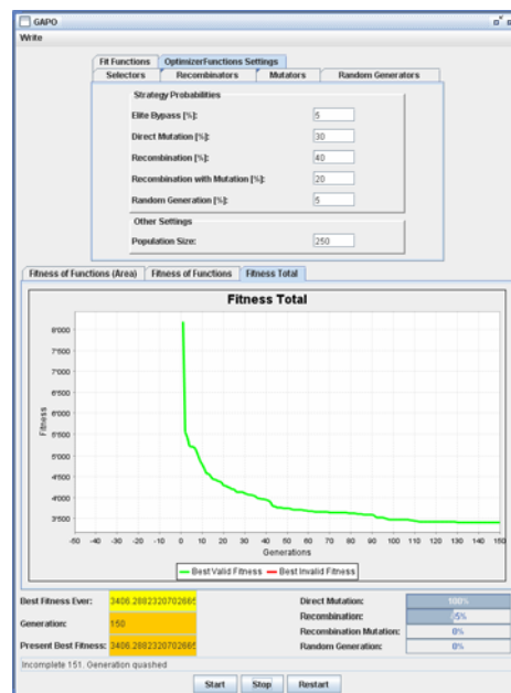
Fig. 2. Screenshot of GAPO's user interface
