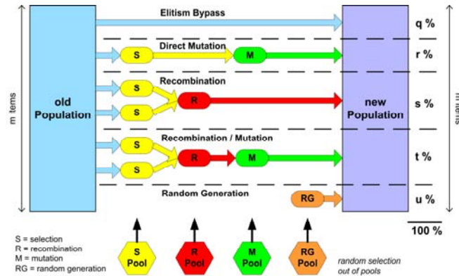
Fig. 1. GAPO Evolution Model
